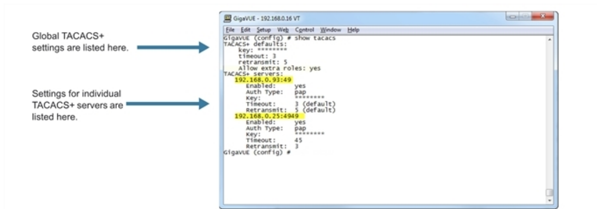
Figure 29 Results of show tacacs Command
